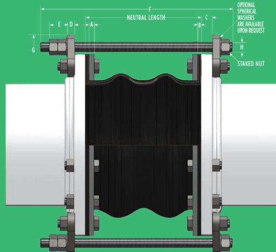
Figure 1 Style 262R
