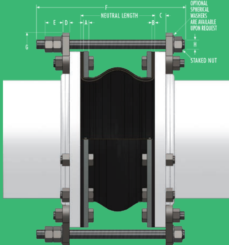
Figure 1 Style 261R
