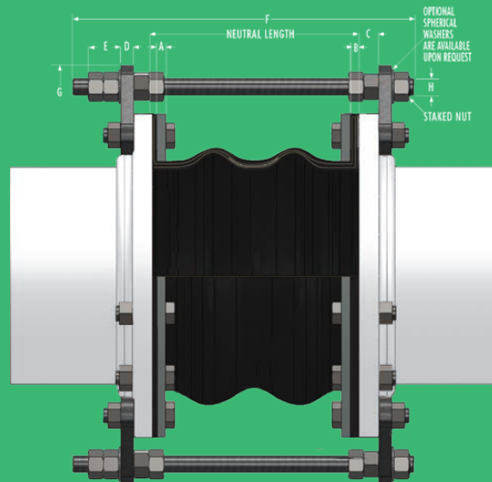
Figure 2 Style 262R
