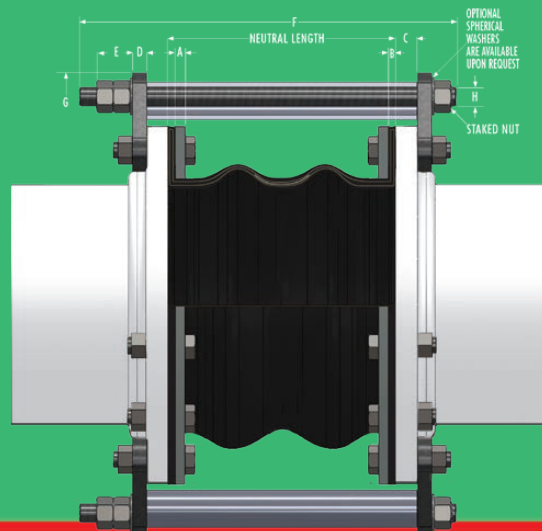
Figure 3 Style 262R
